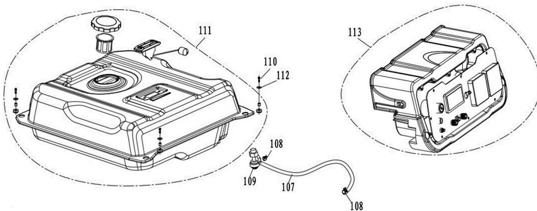
Fig. 28: Spare parts drawing 1 and Spare parts drawing 2 PG-E 40 SRA
