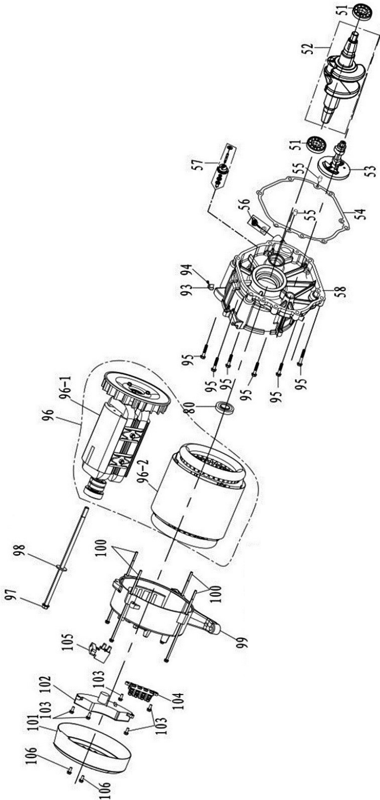
Fig. 29: Spare parts drawing 3 PG-E 40 SRA
