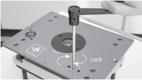
Locking the table in position
