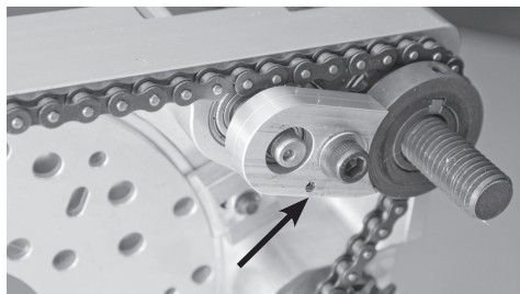
Locking mechanism
