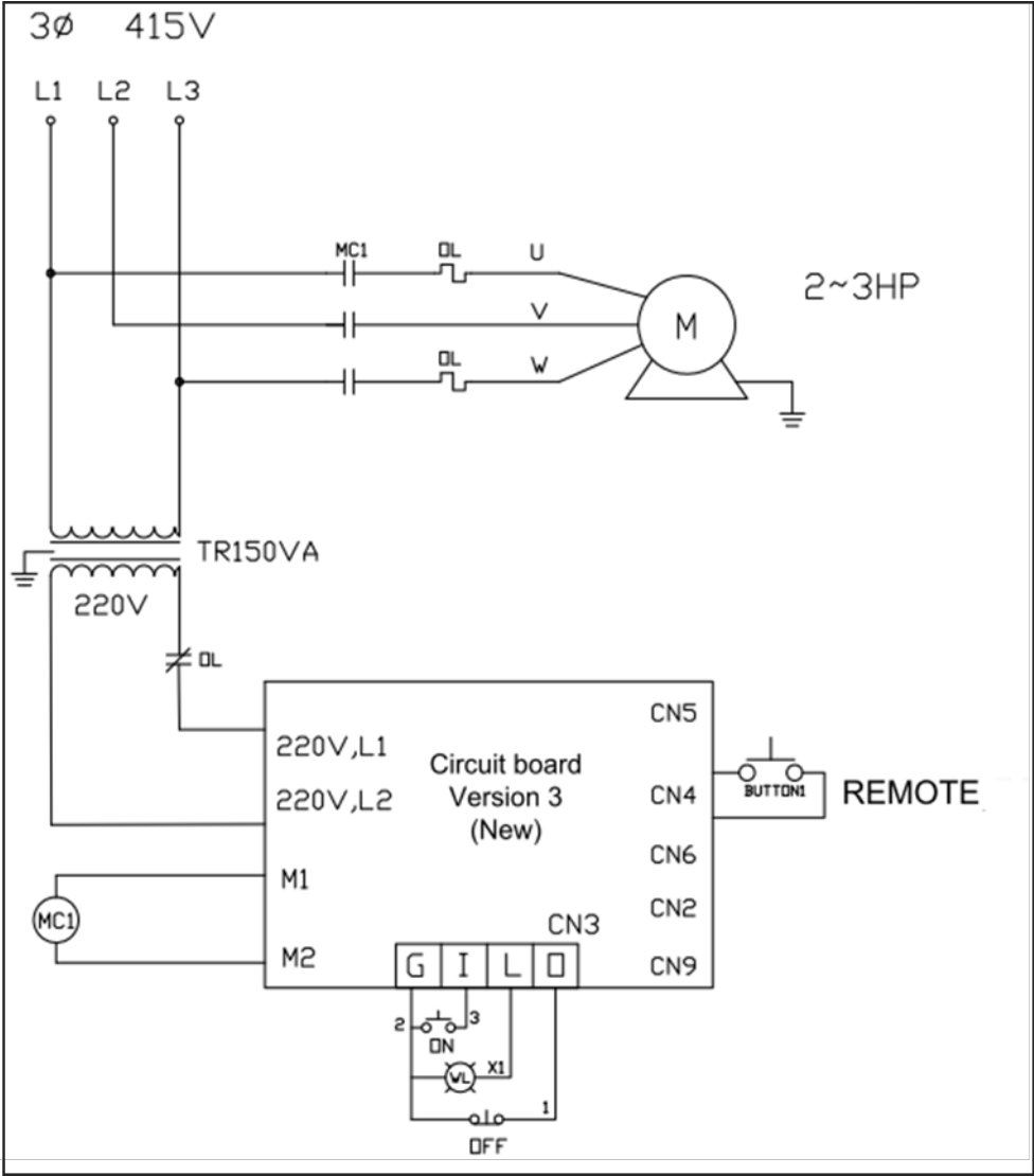
Control panel
