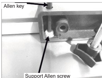
Support Allen screw
