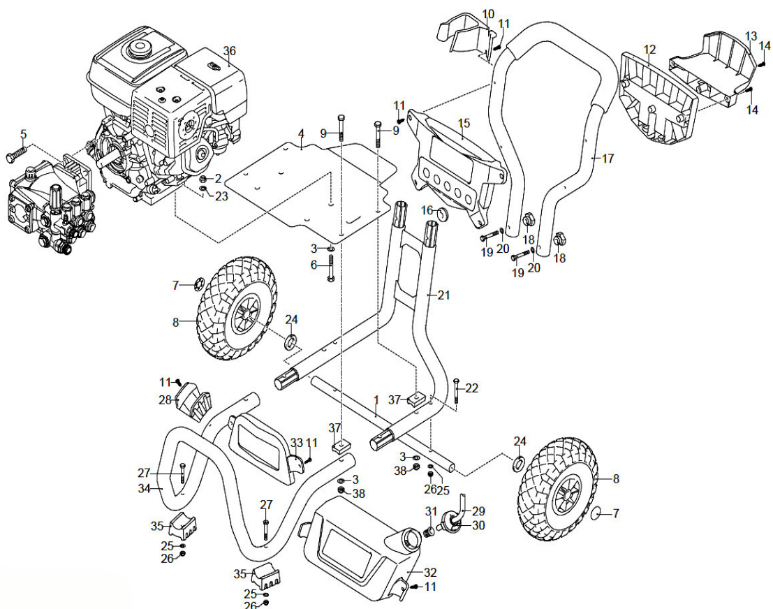
Fig. 15: Spare parts drawing 6 HDR-K 96-28 BL
