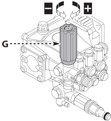
Fig. 10: Adjustment of the working pressure
