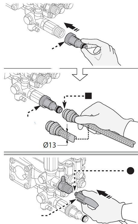
Fig. 6: Water supply
