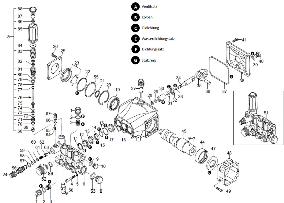
Fig. 13: Spare parts drawing 3 and spare parts drawing 4 HDR-K 72-22 BH
