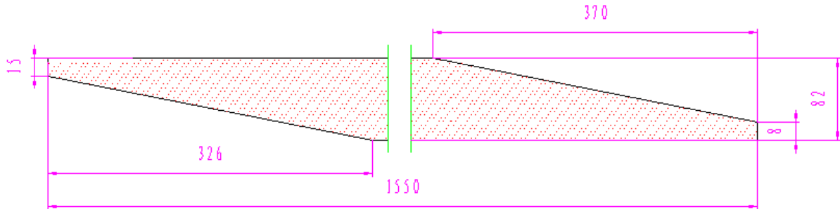
Left Clamp End
