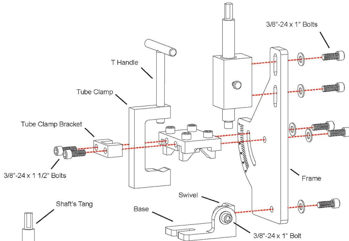
Figure 1 - Exploded View of Complete Notcher
