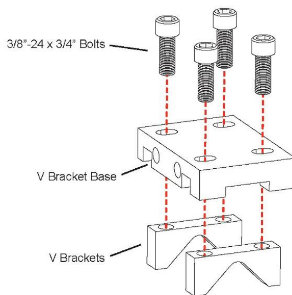
Figure 3 - V-Bracket Assembly
