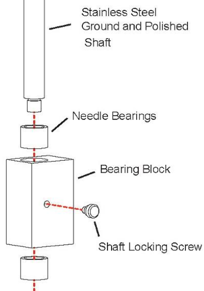
Figure 2 - Shaft and Bearing Block Assembly
