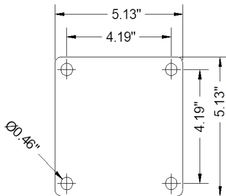
RDB-25 (mounting dimensions)
