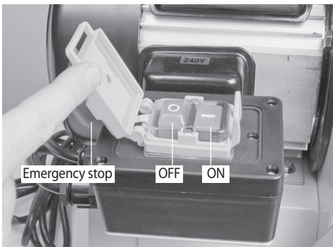
Control Switch
